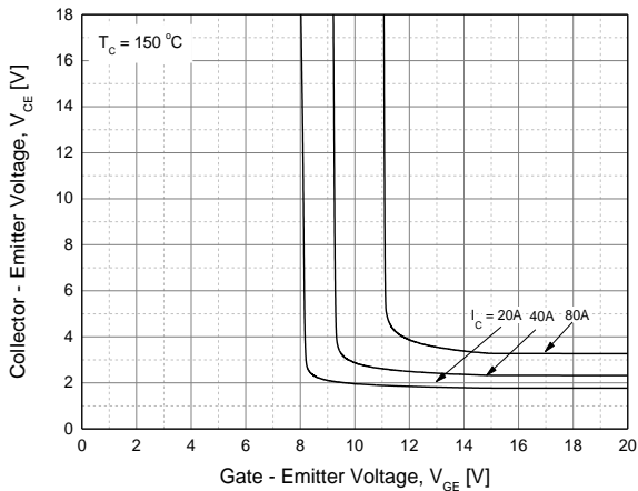
Fig. 5 Saturation voltage vs. gate bias
