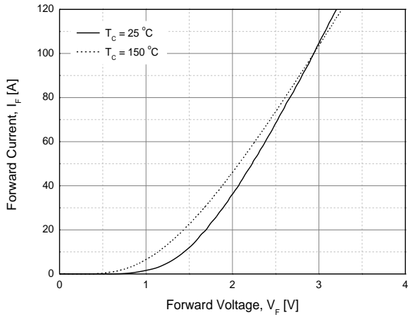
Fig. 18 Conduction characteristics
