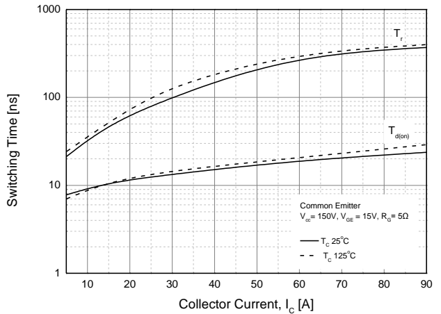
Fig. 8 Turn on time vs. collector current
