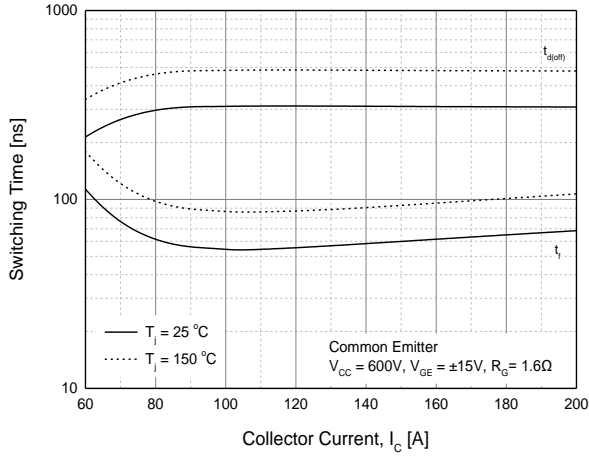
Fig. 7 Turn-off time vs. collector current
